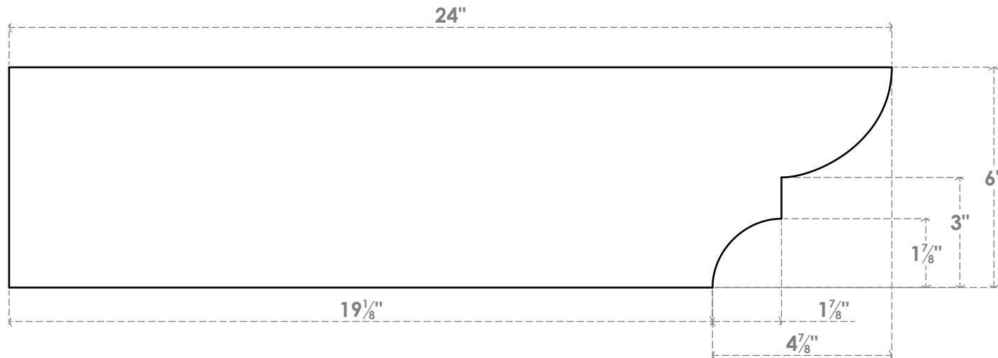
SIDE PROFILE
