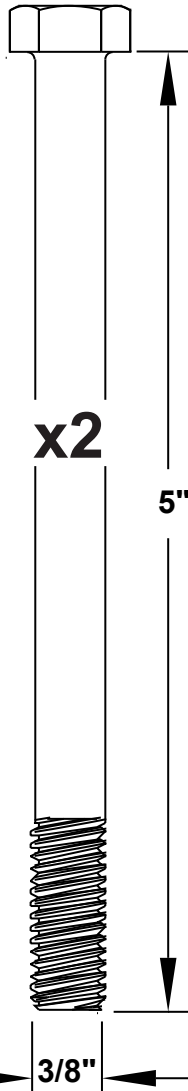
3/8" HEX BOLT
