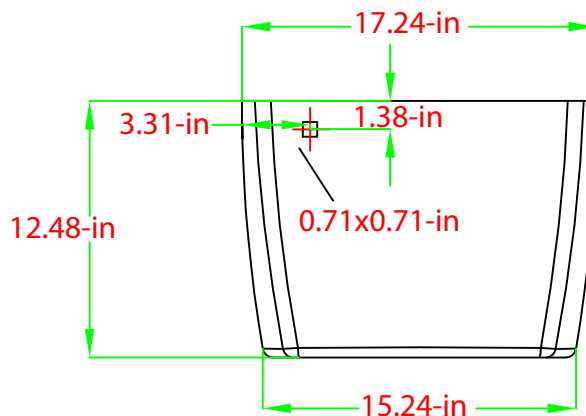
Front View without Lid
