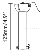
4.Downrod
