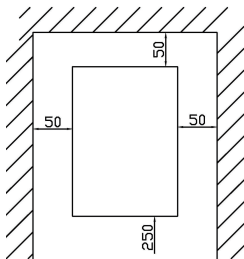
Installation clearance top view (1:10) (mm)
