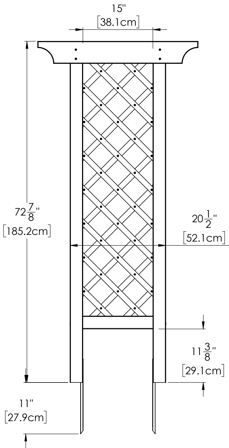
FRONT VIEW
