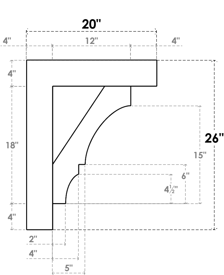
SIDE PROFILE
