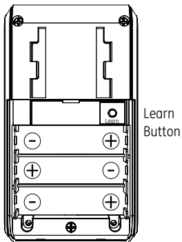
Battery Compartment
