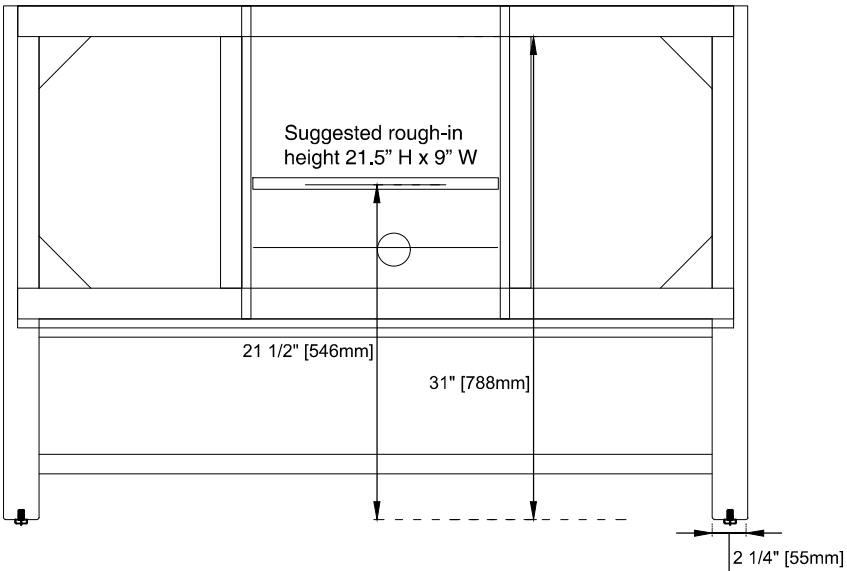
Back View
