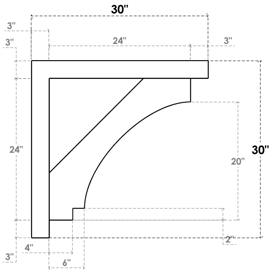
SIDE PROFILE
