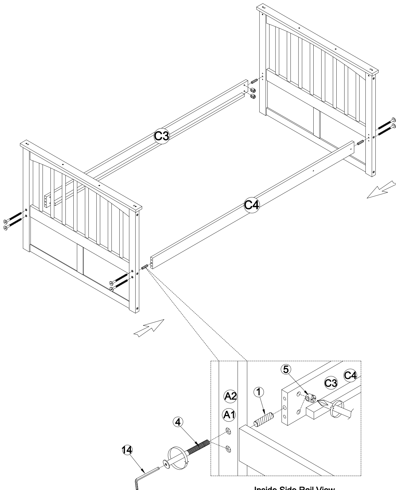
Inside Side Rail View
