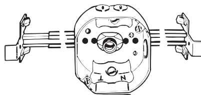
54151-N octagon box mounted on adjustable bar hanger.
