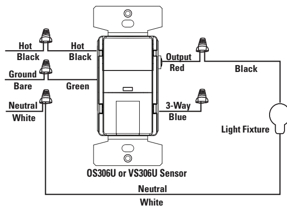
DIAGRAM 2A: SWITCH IN LOCATION WITH HOT WIRE
