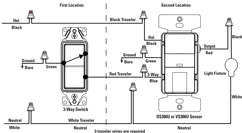
DIAGRAM 2A: SWITCH IN LOCATION WITH HOT WIRE
