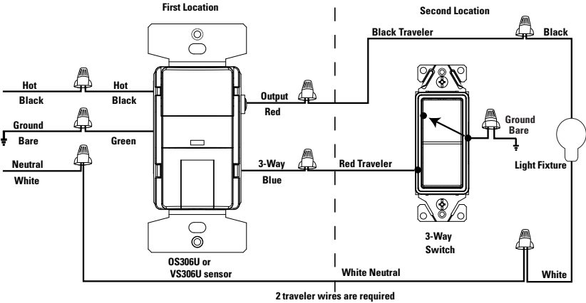
DIAGRAM 3: SENSORS IN BOTH LOCATIONS
