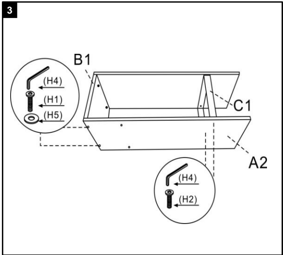
Step 3 Attach the Panel(A2) to Panel(B1),using Allen bolt and washer(H1&H5) Tighten white Allen Key(H4) Attach the Panel(A2) to Metal frame(C1),using Allen bolt(H2) Tighten white Allen Key(H4)
