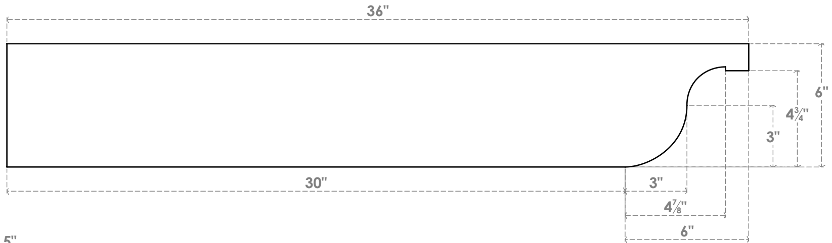
SIDE PROFILE
