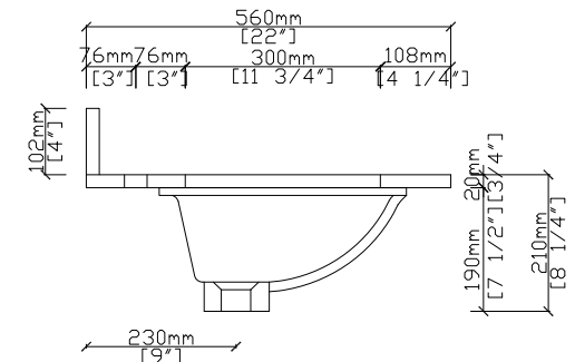
RIGHT VIEW
