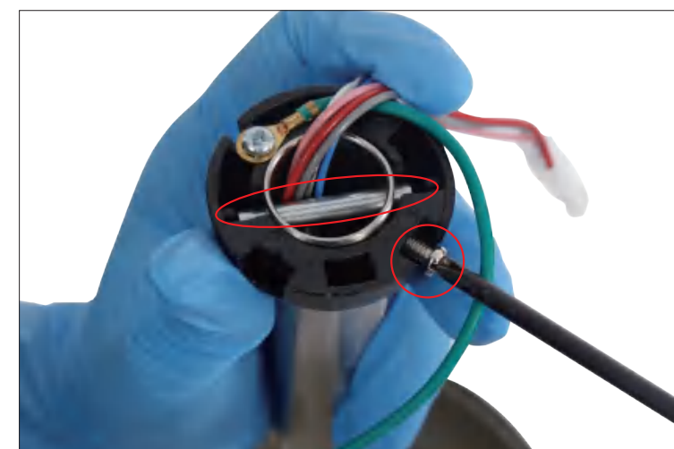
Step 9 Tighten the screws on the hemisphere.
