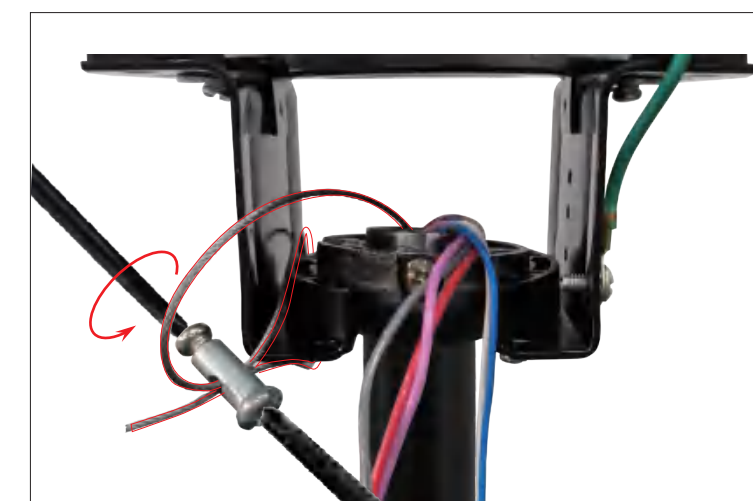
Step 11 Safety rope installation
