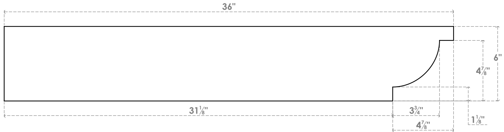
SIDE PROFILE
