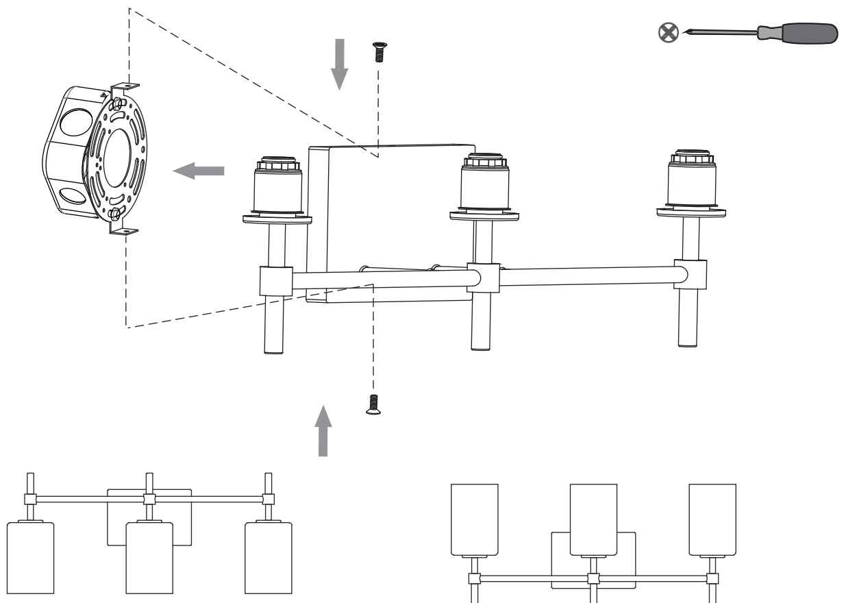
Installation Option 1: Down light
