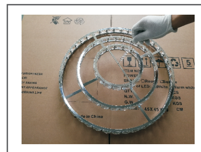
Step 6. Install one end of the crystal chain circular ring in the middle of the lampshade cross-bar hole.
