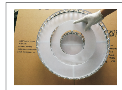
Step 7. Put the acrylic sheet into the lampshade and adjust the position
