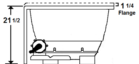
Standard (S) Pump, Blower, & Heater Location
