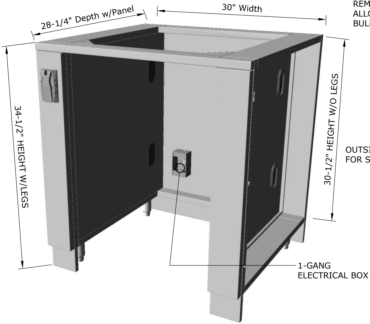
ISO VIEW
