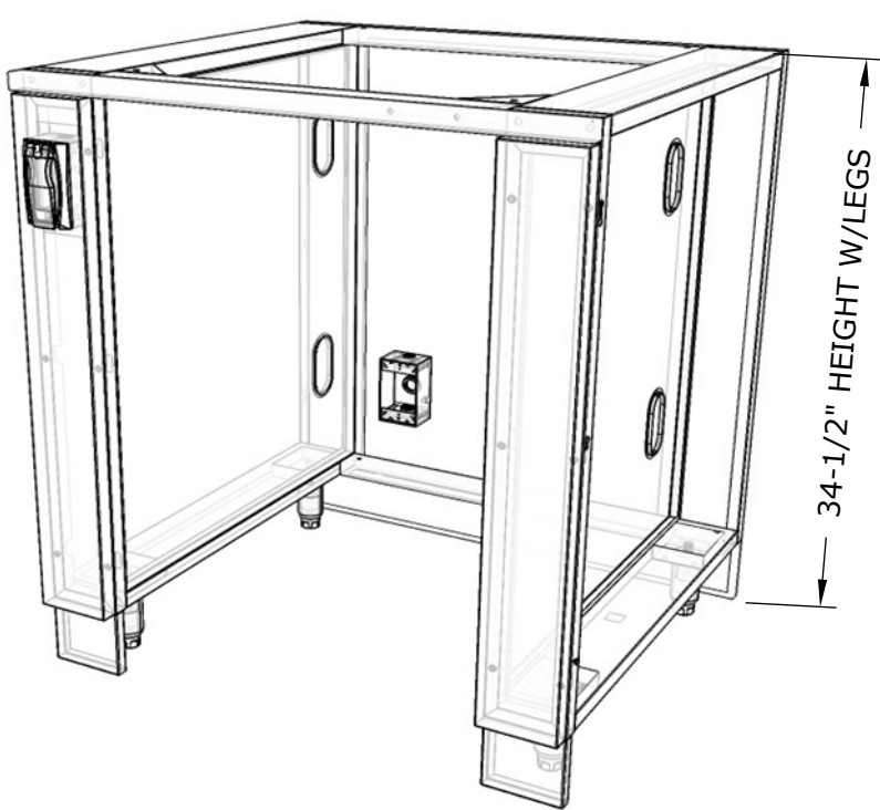
ISO VIEW
