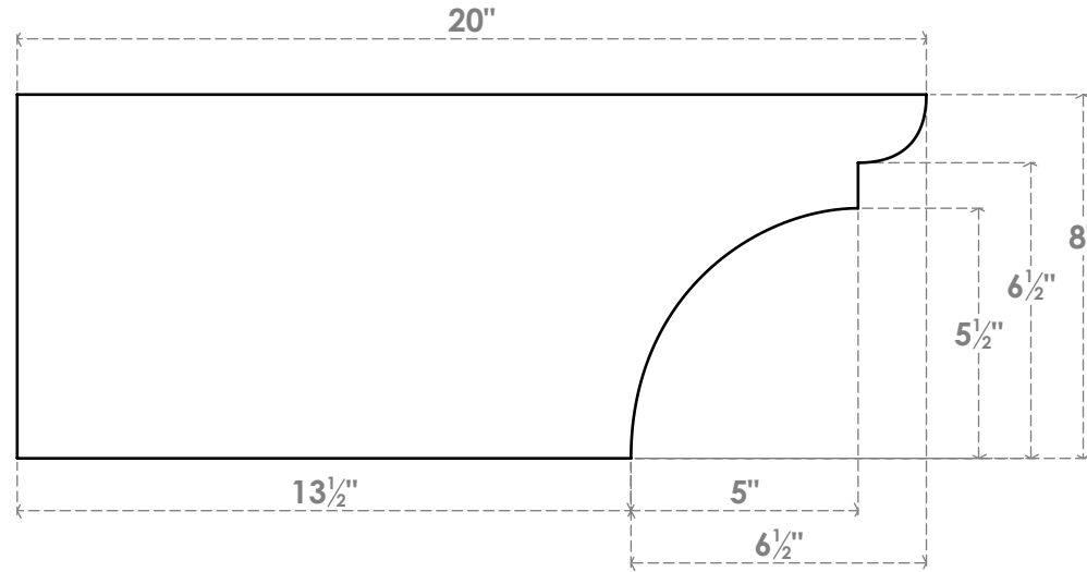
SIDE PROFILE
