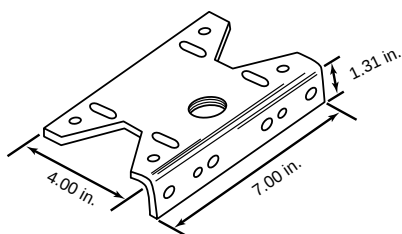
Figure 1: 9049UMS1 Dimensions
