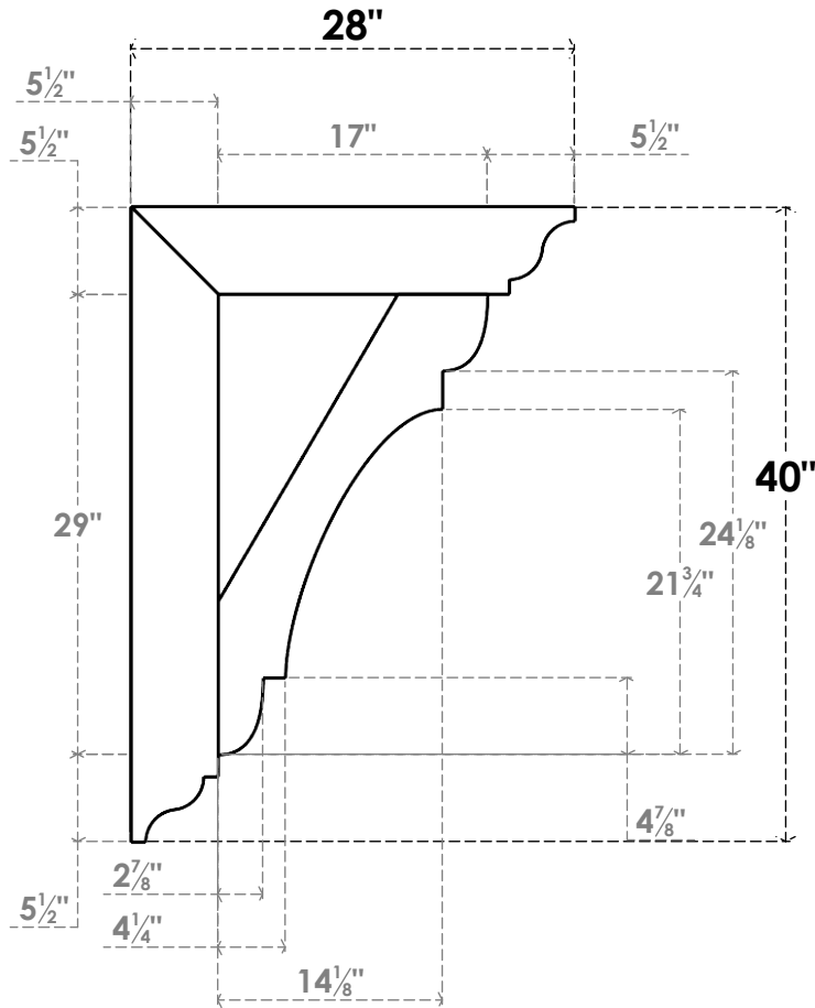
SIDE PROFILE
