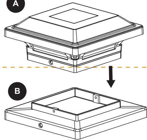
For 6-in x 6-in posts/Para postes de 15,24 cm x 15,24 cm
