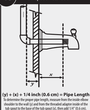
Tub Spout Installation
