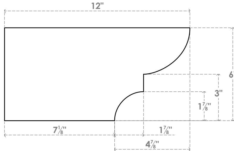
SIDE PROFILE
