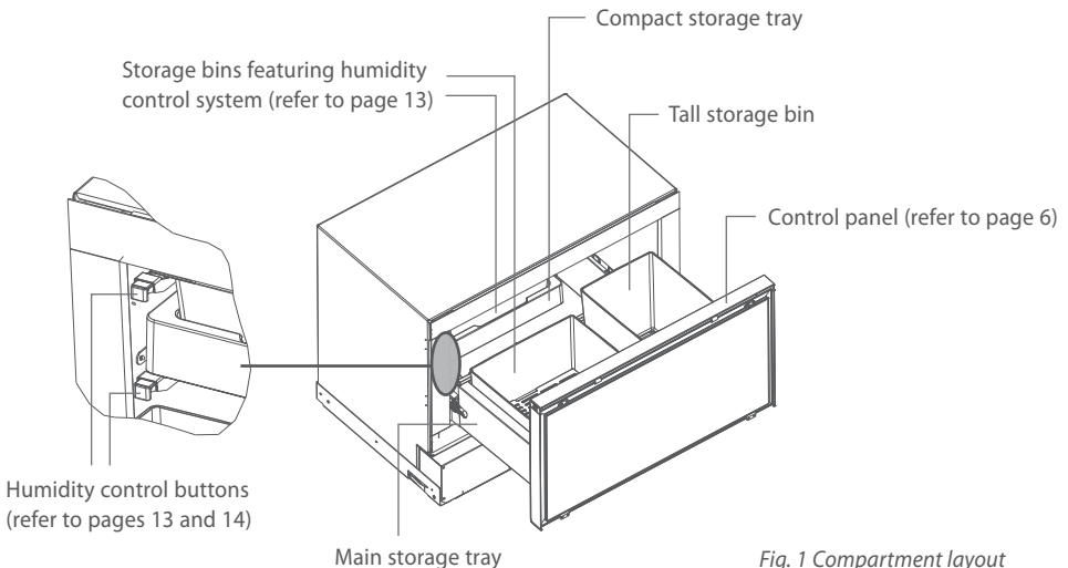
Fig. 1 Compartment layout
