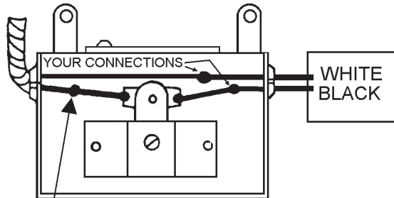
WIRING THE THERMOSTAT CONECTANDO EL TERMOSTATO
