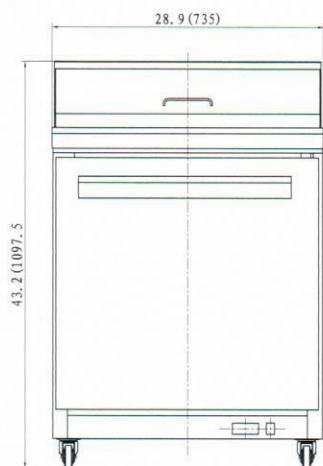
MXCR-29S
