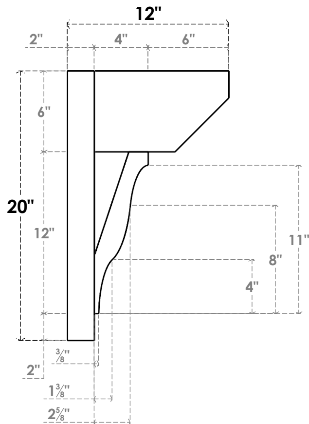
SIDE PROFILE
