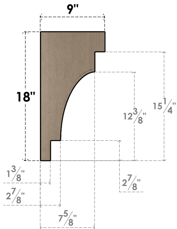
SIDE PROFILE
