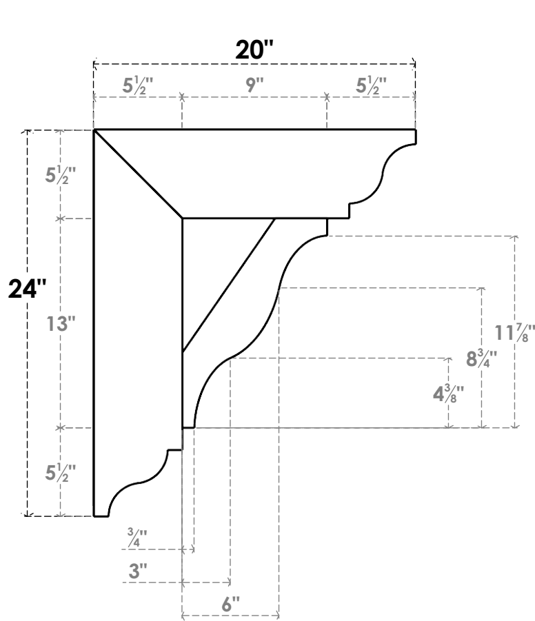
SIDE PROFILE
