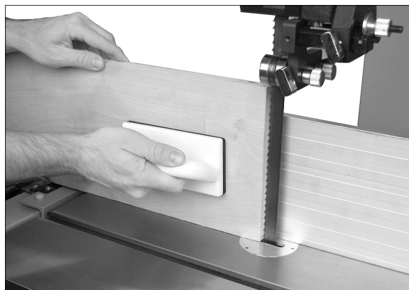
Figure 40 (resawing)
