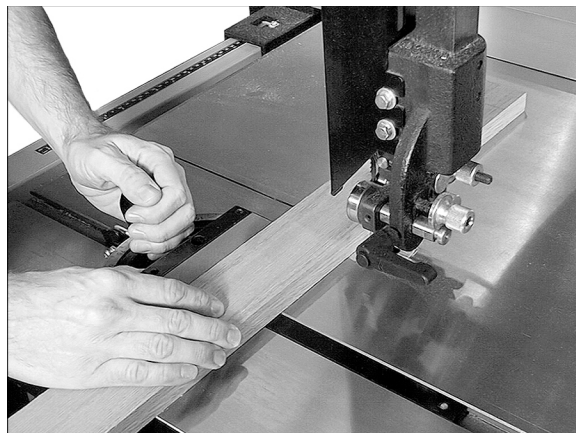
Figure 39 (crosscut)
