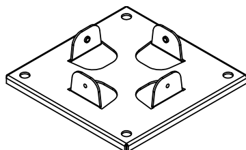
P1 | A4M01454 (x4) | POST FOOT
