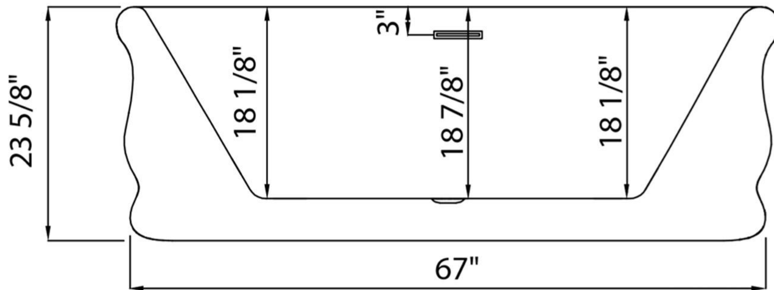
FRONT VIEW
