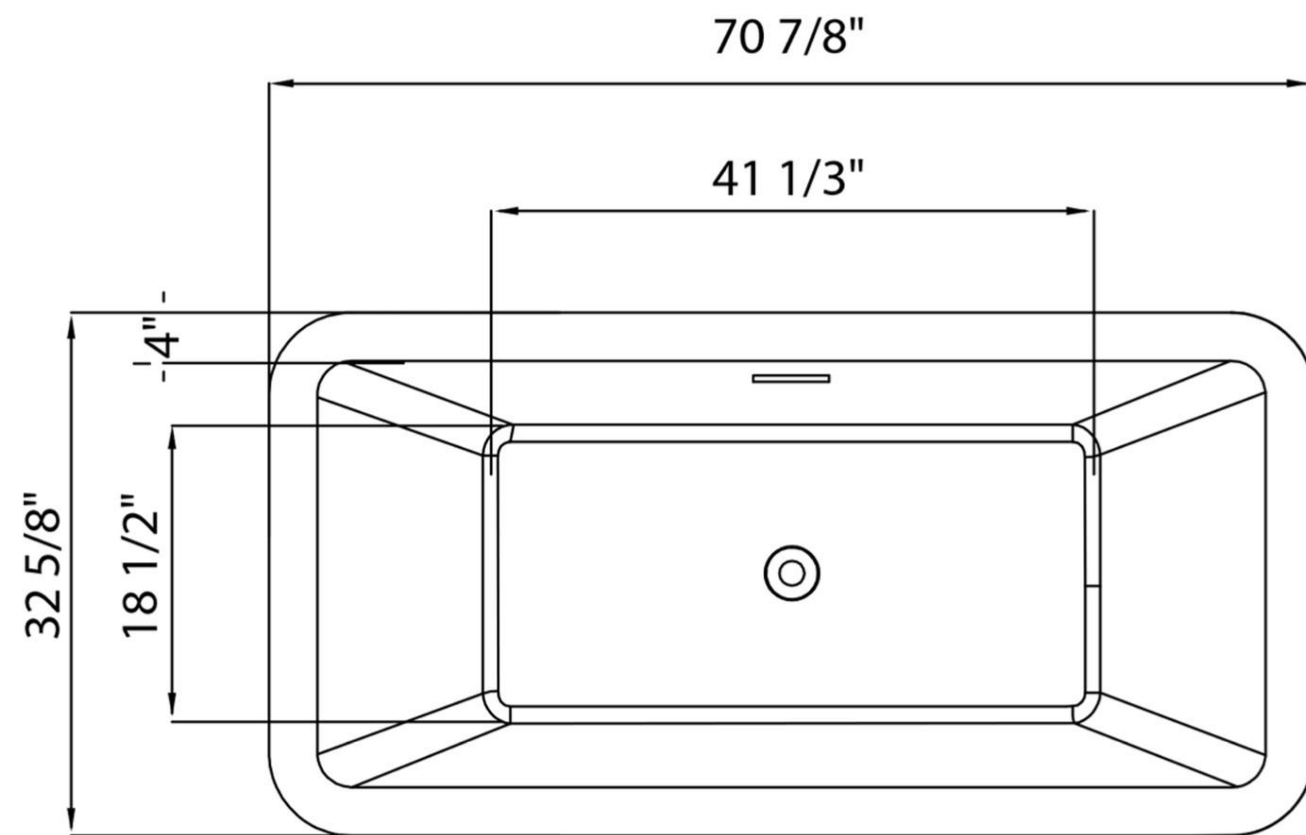
TOP VIEW
