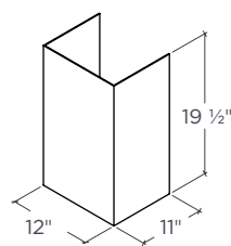
LOWER CHIMNEY COVER
