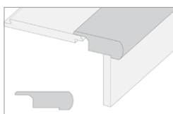
9/16" Overlap Stair Nosing
