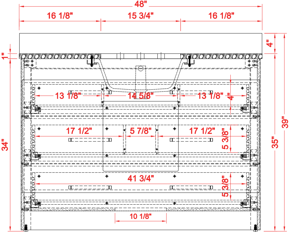
BACK VIEW
