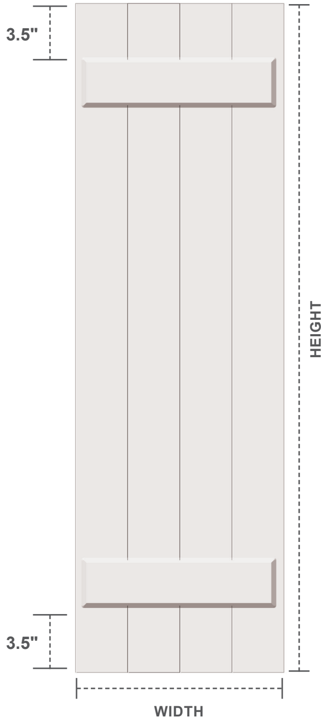
FRONT VIEW
