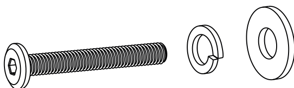
ALLEN KEY BOLT: M6 X 50mm - QTY 8 LOCK WASHER: \varnothing 10 / \varnothing 6 X 1.5mm - QTY 8 WASHER: \varnothing 16 / \varnothing 6 X 1mm - QTY 8 QTY 8 SETS
