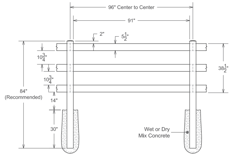
3-Rail
