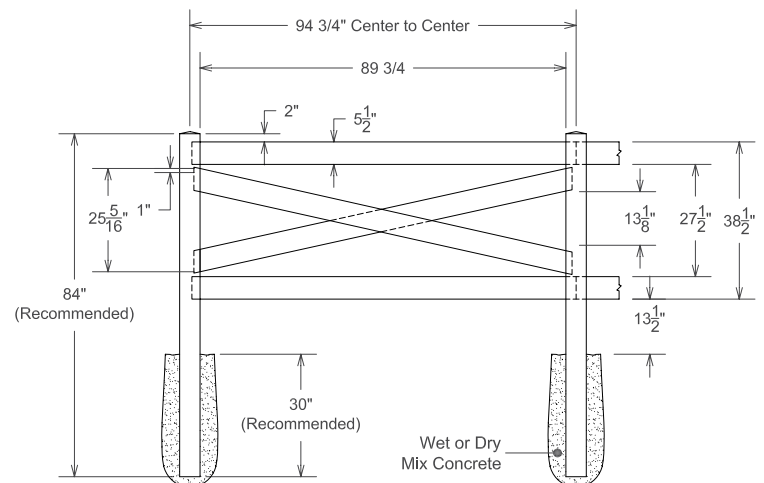
Crossbuck
