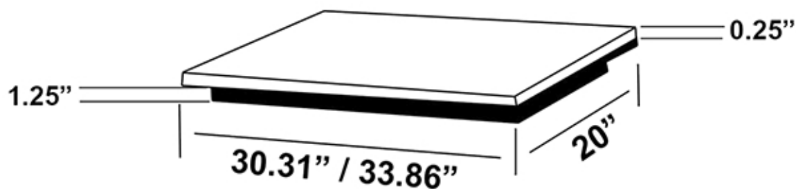
CUT-OUT VIEW
