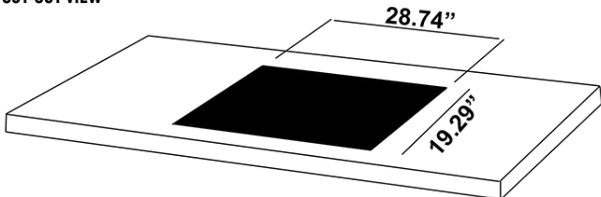
CUT-OUT VIEW
