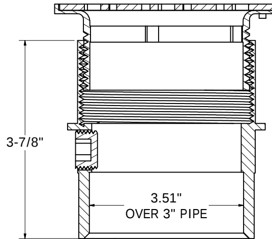
SECTION A-A SCALE .9
