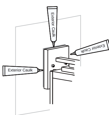
Rectangle/Square Backplate
