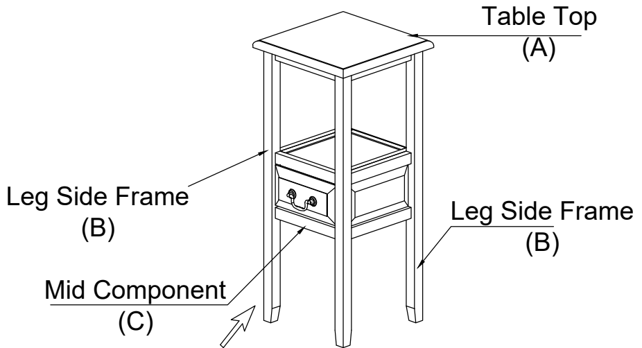
FRONT FACING
