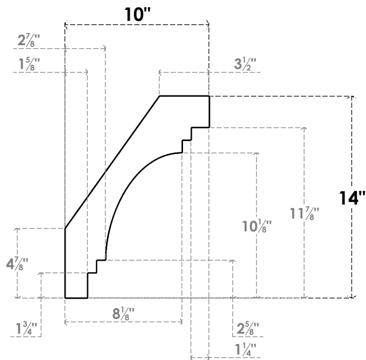
SIDE PROFILE
