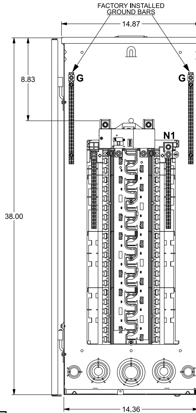
PNW4040B1200C Main Breaker Load Center
