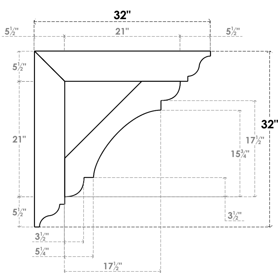
SIDE PROFILE
